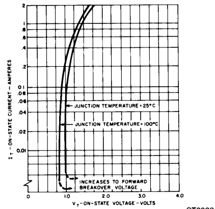
Figure 12. On-State Characteristics
